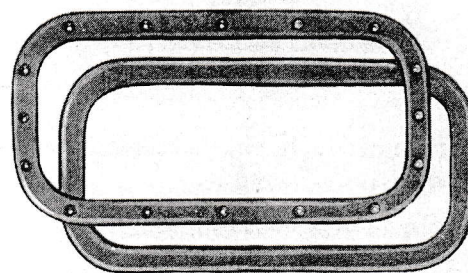
No. 135 RECTANGULAR SHAPE I.D. 7" x 16" O.D. 9" x 18"
