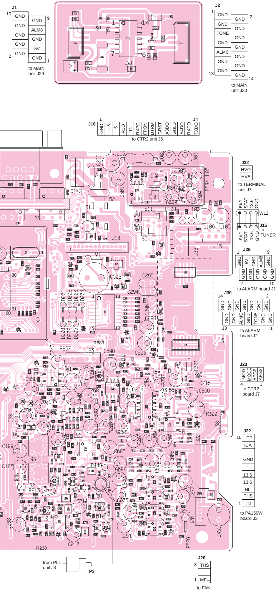
8-2-5 ALARM BOARD
