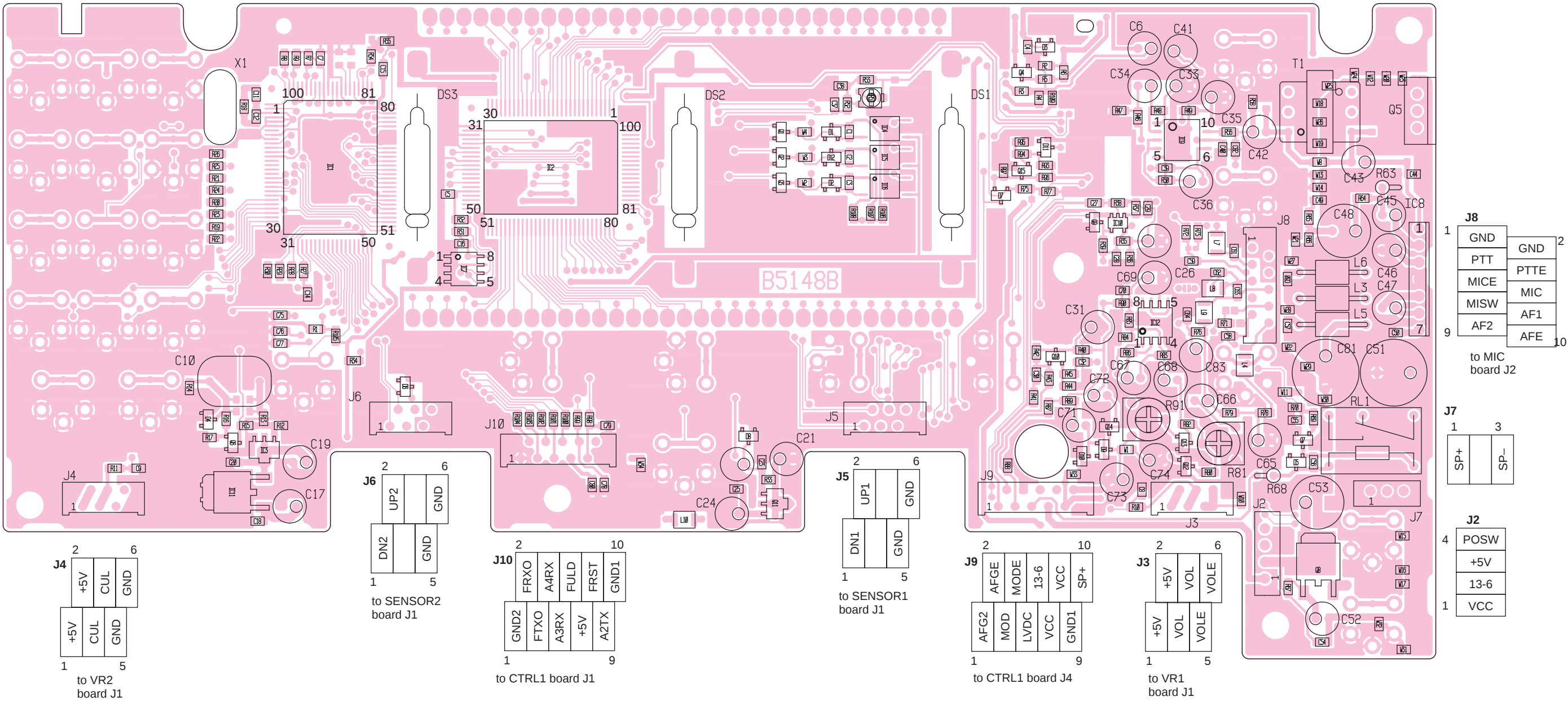
8-1 RC-21 8-1-1 LOGIC BOARD • TOP VIEW
